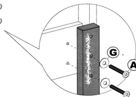
Low bedhead assembly method
